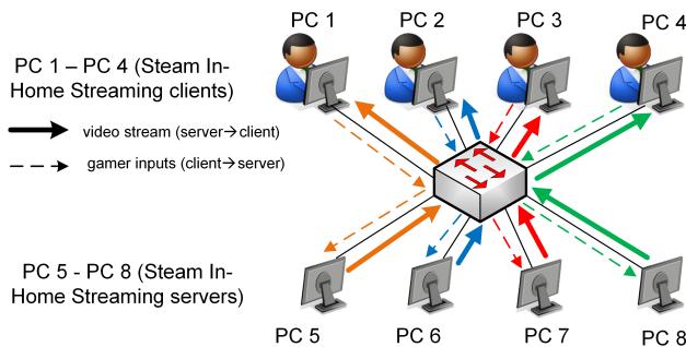
Figure 1: Laboratory testbed
