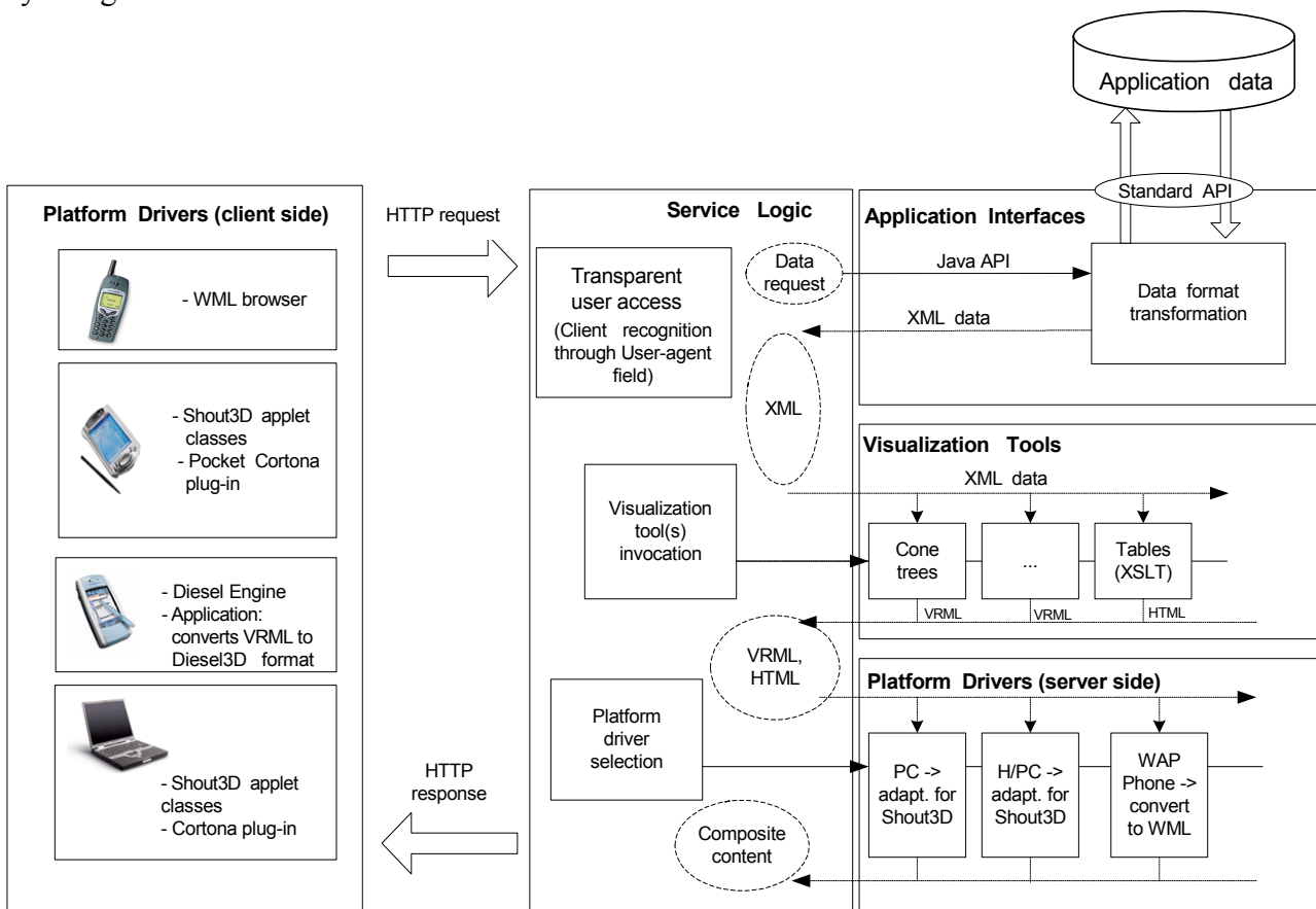
Figure 2. MUVA system architecture
