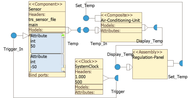
Figure 1. SaveCCM model of Temperature regulation system
