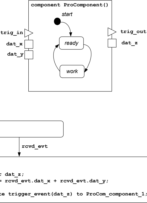
Figure 7.1 Example of a theoretical state chart for a ProCom component
